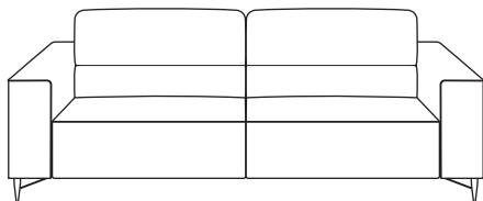
Large Sofa (5391-64) W:226 x D:100 x H:98cm SW:90 x SD:55 x SH:49cm
